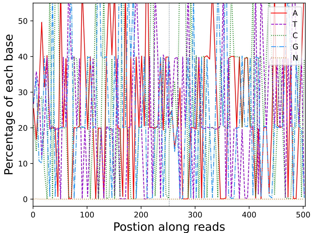
Base percentage along reads (R10204)
